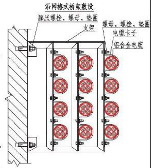
铝合金电缆在竖井内多层敷设
